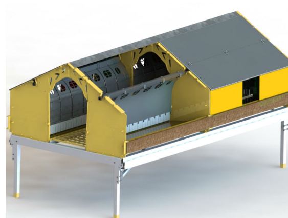
Example of a breeder house equipped with the Breedio breeder nest
